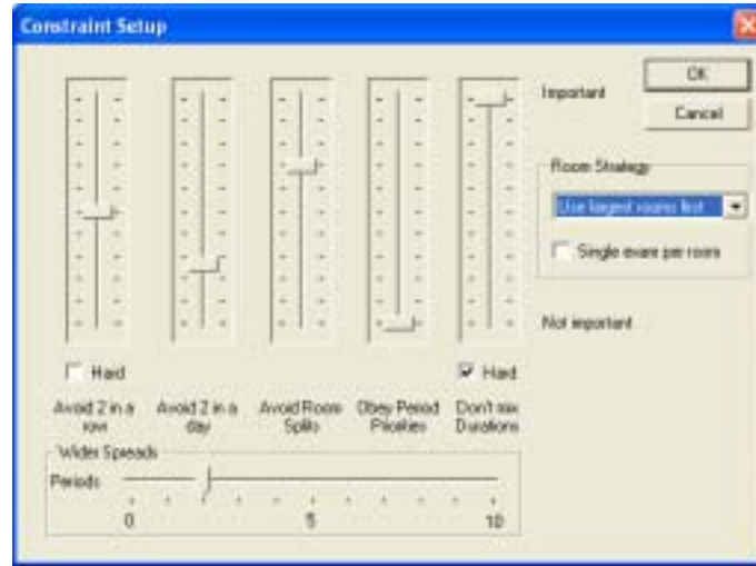
Figure 4 – Optimisation Constraints
